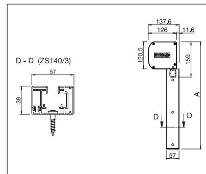
VS5200 Soffit mounting
